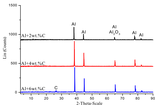
Fig. 3 XRD patterns of activated carbon and composites
