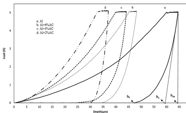
Fig. 5 Graph of loading–unloading/depth of activated carbons added to pure Al and Al in different
