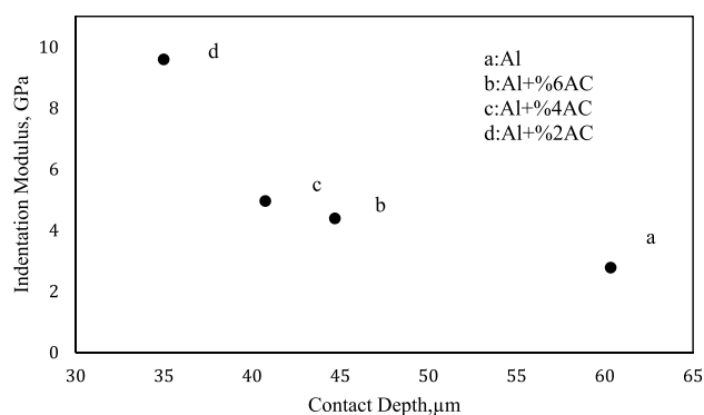
Fig. 6 Elastic modulus values obtained from dynamic hardness test
