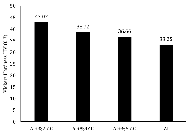
Fig. 4 Hardness values obtained by adding different activated carbon quantities to pure Al
