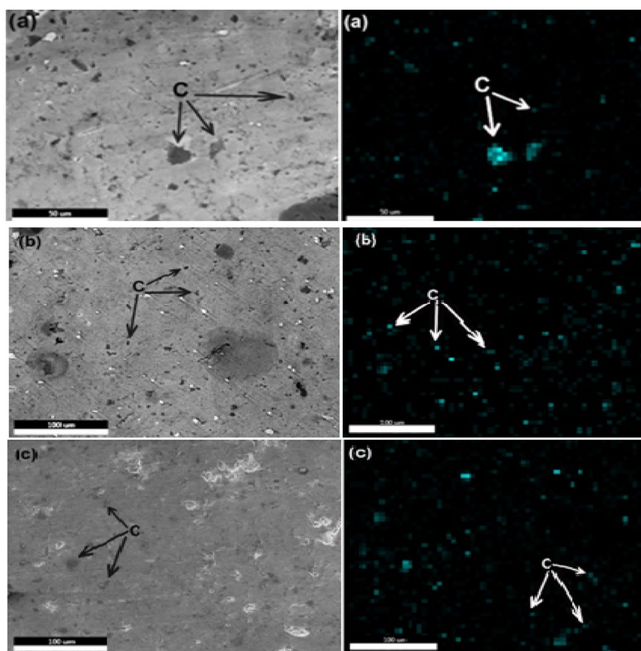
Fig. 1 SEM image and Energy dispersive spectrometer measurement (EDS) from these phases are given of Al–AC composites: (a) 2% AC, (b) 4% AC, (c) 6% AC
