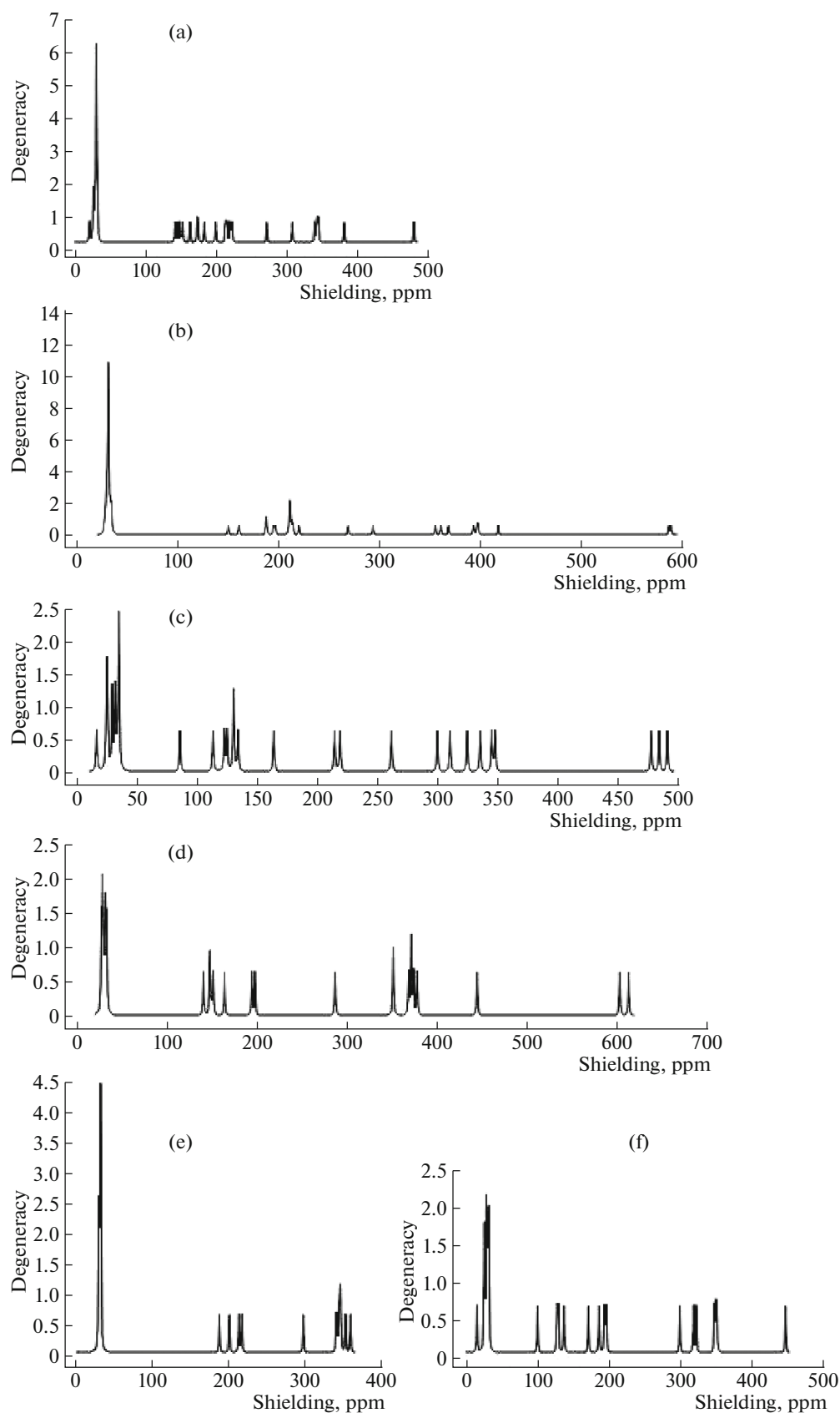
Fig. 3. The ^1\text{H} -NMR of (a) 5AEL- \text{Mg}^{2+} , (b) 5AFX- \text{Mg}^{2+} , (c) 4QPF- \text{Ca}^{2+} , (d) 3DYG- \text{Ca}^{2+} , (e) 2F92- \text{Sr}^{2+} , and (f) 2I19- \text{Sr}^{2+} using SCF GIAO method NMR due to B3LYP function and 6-311+G(2d,p) basis set for metal cations of \text{Mg}^{2+} , \text{Ca}^{2+} , \text{Sr}^{2+} , and 6-311+G(2d,p) basis set for other elements.
