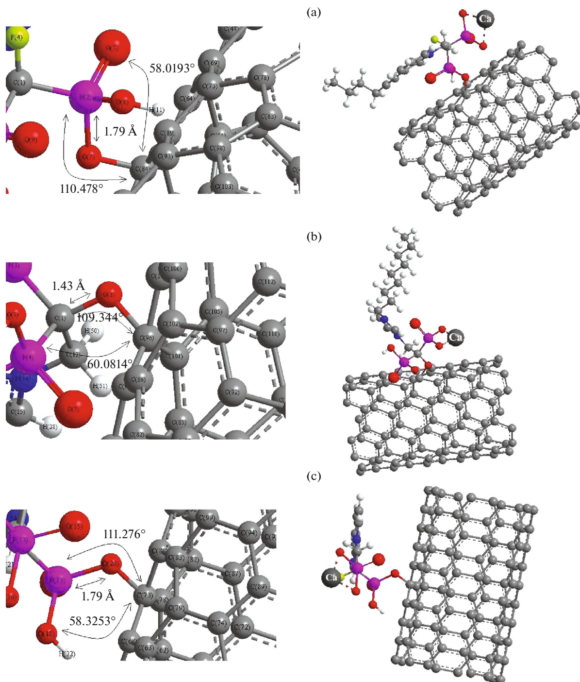
Fig. 1. Adsorption of (a) 5AEL, (b) 5AFX, (c) 4QPF, (d) 3DYG, (e) 2F92, (f) 2I19 chelated with \text{Ca}^{2+} onto surface of (5,5) arm-chair CNT.
