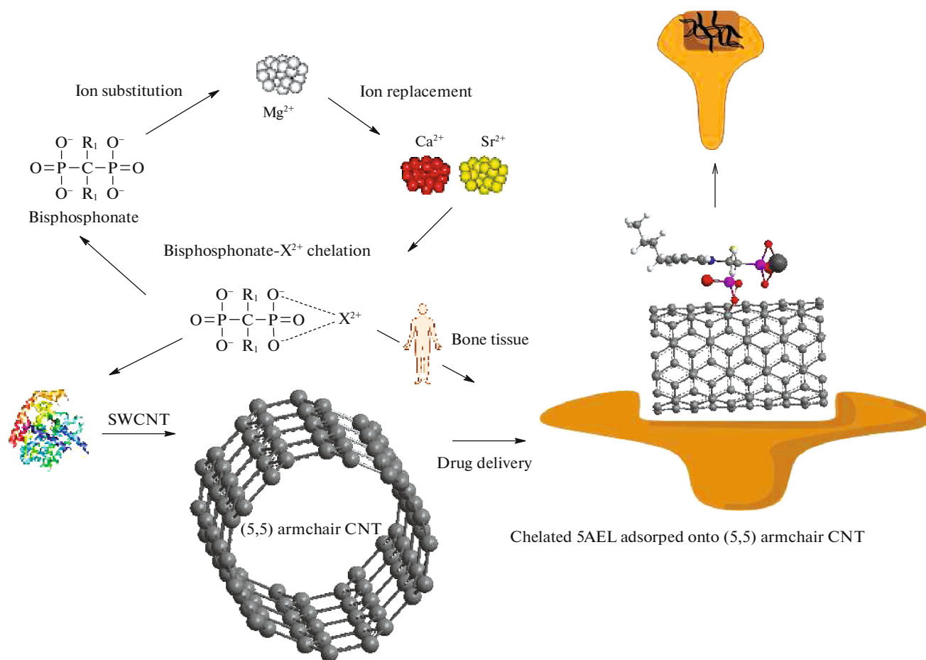
Scheme 2. Drug delivery of (5,5) armchair-SWCNT jointed with bisphosphonate agents of 5AEL, 5AFX, 4QPF, 3DYG, 2F92, 2I19 chelated with Mg 2+ , Ca 2+ , Sr 2+ in the bone of human body.
