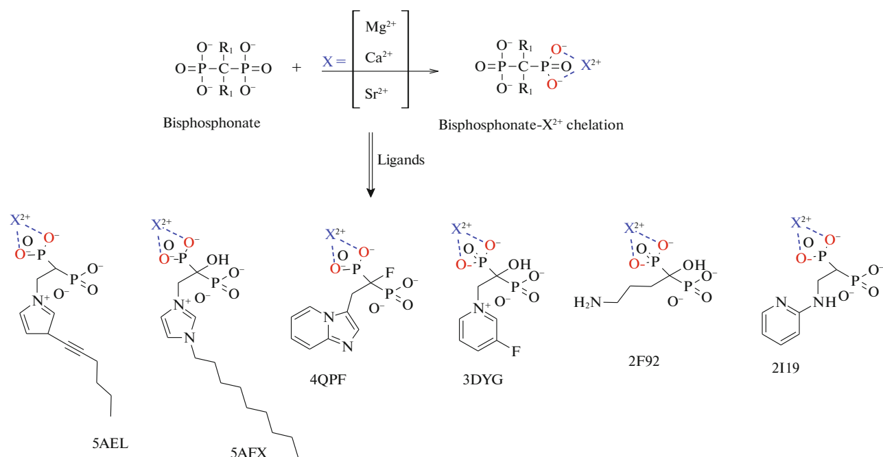
Scheme 1. Proposed mechanism of bisphosphonate–metal cation chelation of \text{Mg}^{2+}/\text{Ca}^{2+}/\text{Sr}^{2+} through the \text{O}^- of two \text{PO}_3 (phosphonate) groups covalently linked to carbon for six ligands of 5AEL, 5AFX, 4QPF, 3DYG, 2F92, and 2I19.
