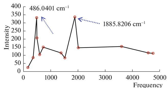
Fig. 5. Calculated IR intensity (km/mol) versus frequency ( \text{cm}^{-1} ) for 4QPF- \text{Ca}^{2+} bisphosphonate agent adsorbed onto (5,5) armchair SWCNT using 6-311+G(2d, p) calculations.
