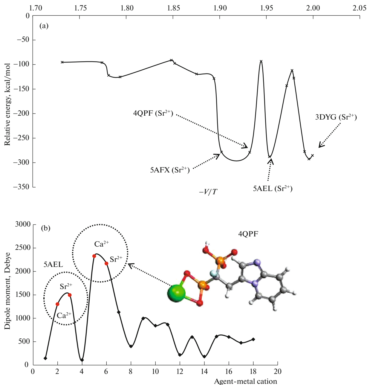
Fig. 6. (a) Relative energy versus virial coefficient ( -V/T ), (b) dipole moment changes for chelated agents of 5AEL, 5AFX, 4QPF, 3DYG, 2F92, 2I19 with each metal cations of \text{Mg}^{2+} , \text{Ca}^{2+} , and \text{Sr}^{2+} adsorbed onto (5,5)-SWCNT.
