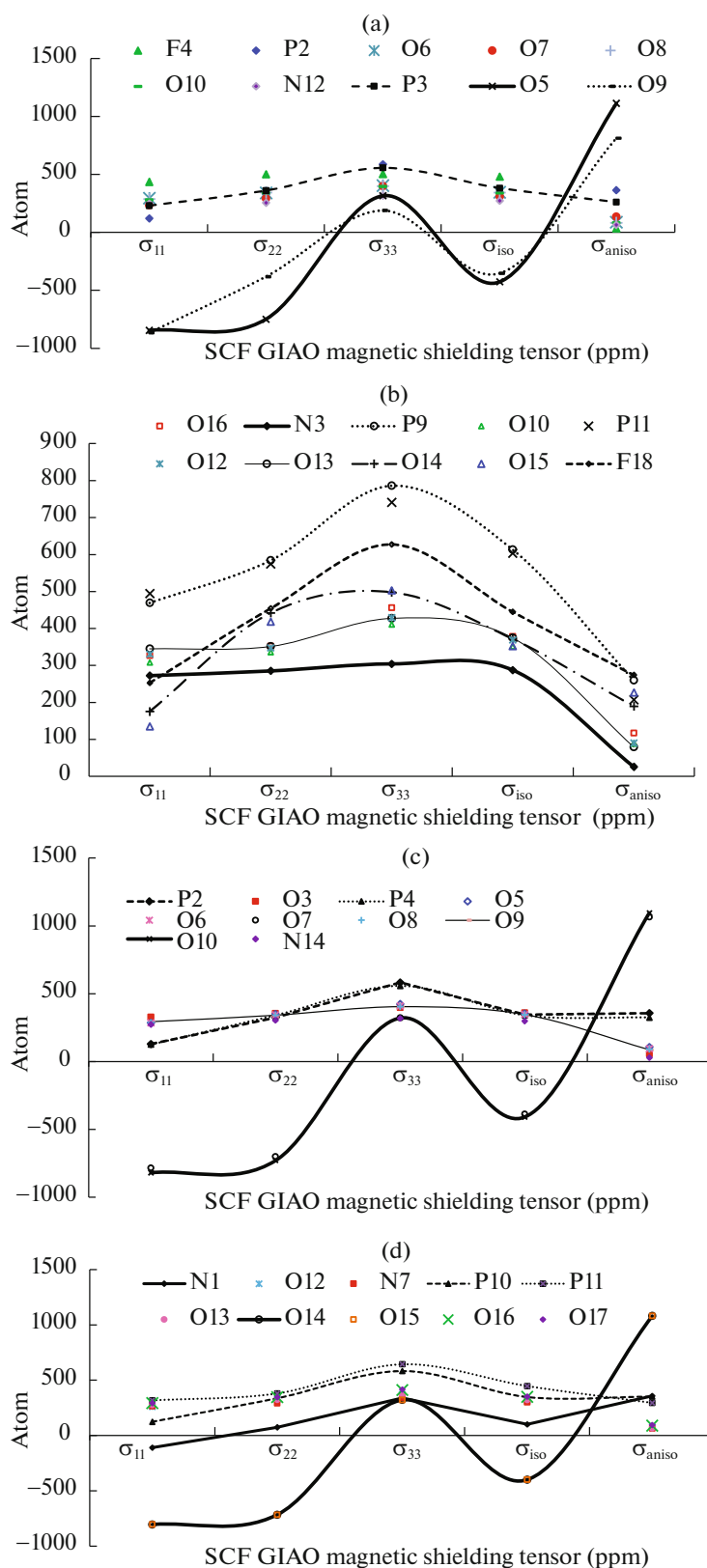
Fig. 2. The ^{13}\text{C} -NMR shifts of isotropic ( \sigma_{\text{iso}} ), anisotropic ( \sigma_{\text{aniso}} ), and eigenvalue shielding tensors ( \sigma_{11} , \sigma_{22} , \sigma_{33} ) calculated by level of theory B3LYP/6-311+G(2d, p) for (a) 5AEL and similar behavior of 4PF; (b) 3DYG and similar behavior for 5AFX in ppm adsorbed site onto (5,5) armchair SWCNT; (c) 2F92 and (d) 2119 through electronegative atoms of N, O, P, and F as the active positions in the structures of bisphosphonate agents.
