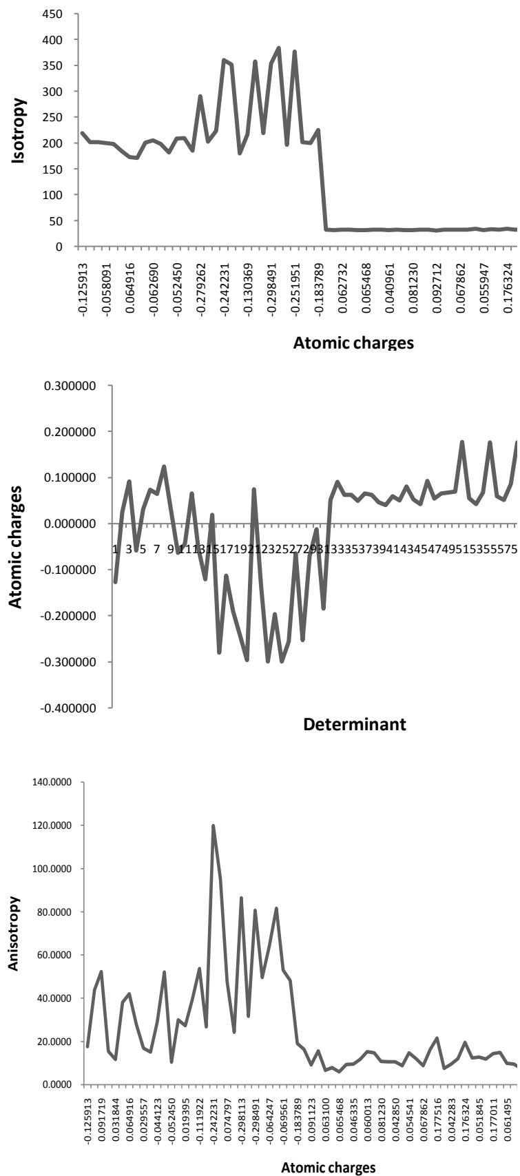
Figure 1. It shows the graphs were obtained from HF/Sto-3G method.
