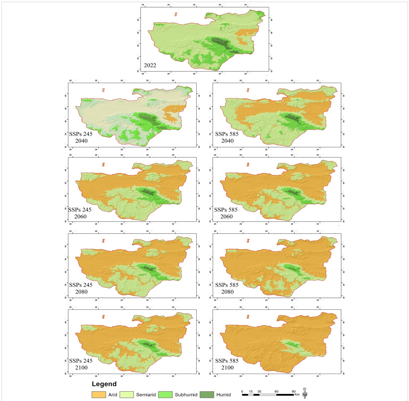
Figure 3. Alteration of Climate Classification Based on the Erinç Climate Classes.
