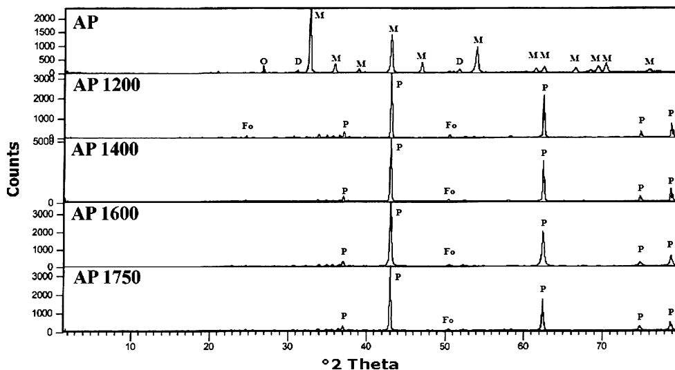
Figure 7. X-ray diffraction patterns of AP samples heated at different temperatures (M: magnesite, D: dolomite, O: olivine, P: periclase, Fo: forsterite).
