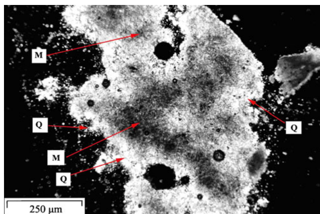
Figure 2. Polarized light micrograph of a magnesite particle containing cryptocrystalline quartzite.
