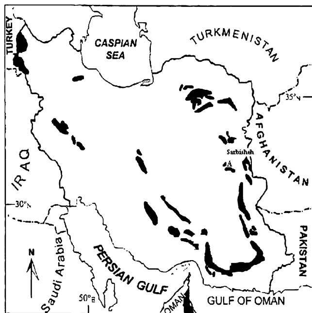
Figure 1. Index map showing the locations of major Iranian ophiolites and the location of Afzal Abad magnesite deposit studied in this investigation (A: Afzal Abad mine).
