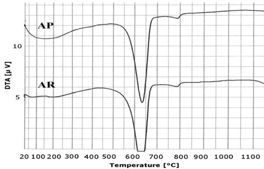
Figure 5. DTA curves of AR (as-received) and AP (processed) samples.
