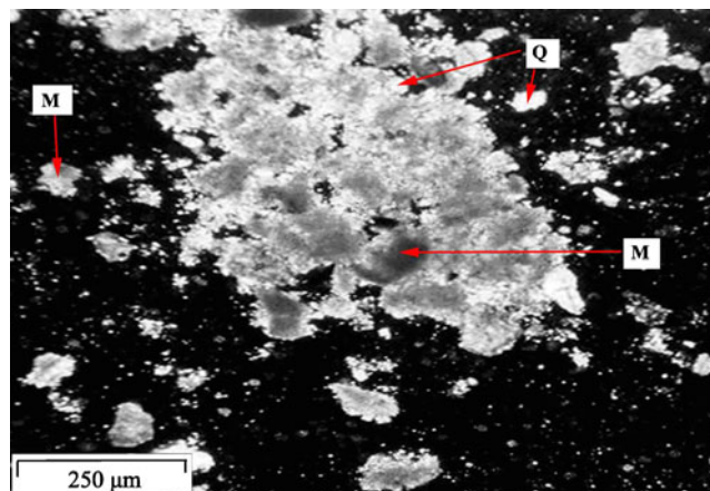
Figure 3. Polarized light micrograph of free magnesite particles after crushing (75 \mu\text{m} ) accompanied by quartzite particles.
