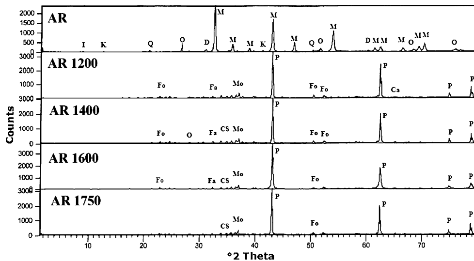
Figure 6. X-ray diffraction patterns of AR samples heated at different temperatures (M: magnesite, D: dolomite, O: olivine, Q: quartzite, K: kaolinite, I: illite, P: periclase, Fo: forsterite, Mo: monticellite, Ca: calcium oxide, Fa: fayalite, CS: calcium silicate).
