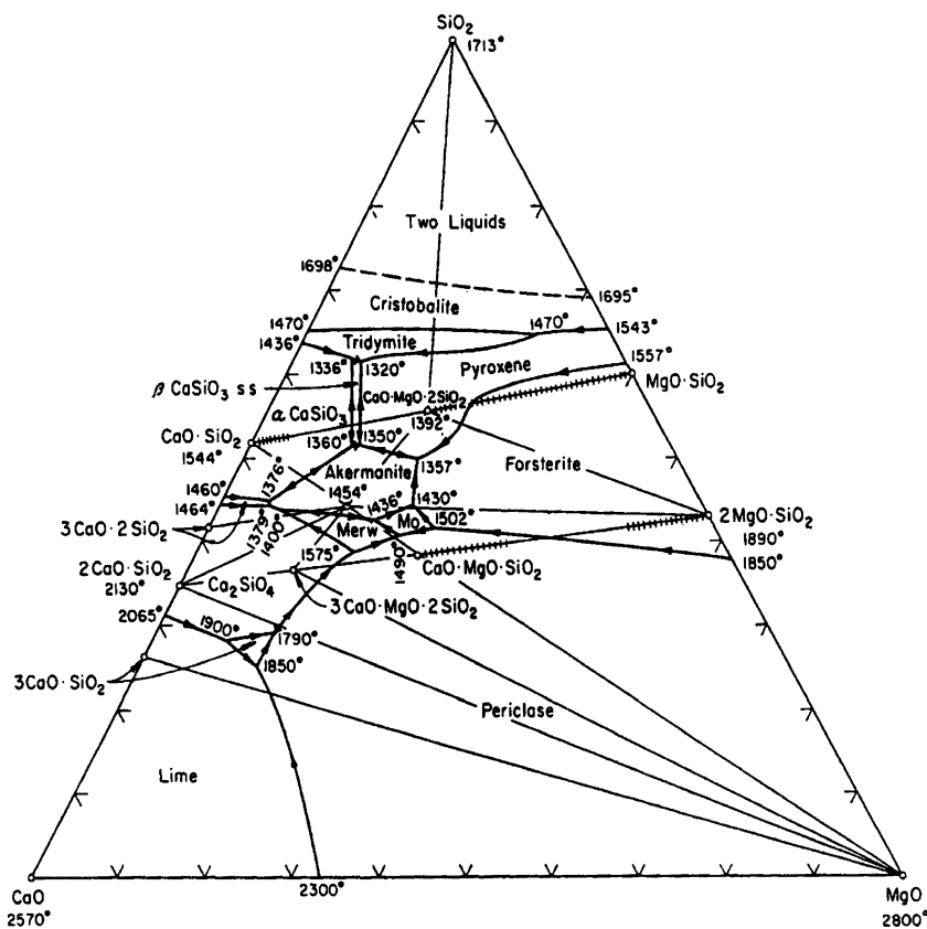
Figure 8. MgO-SiO 2 -CaO ternary phase diagram.
