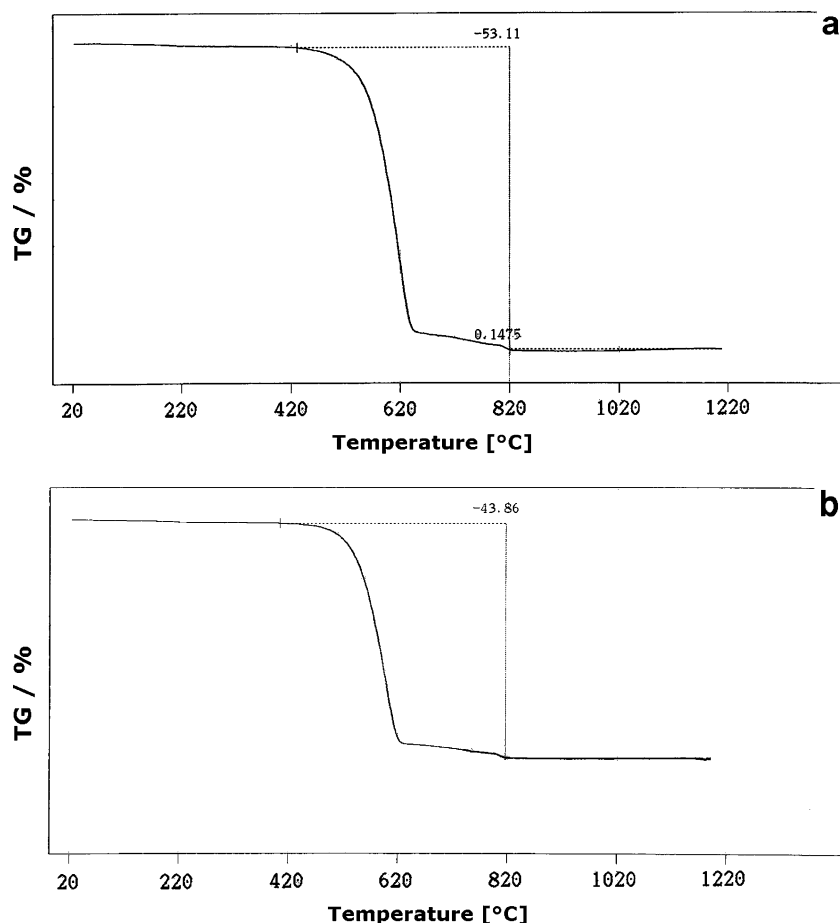
Figure 4. TG curves of magnesite ore samples: (a) As-received and (b) processed sample.
