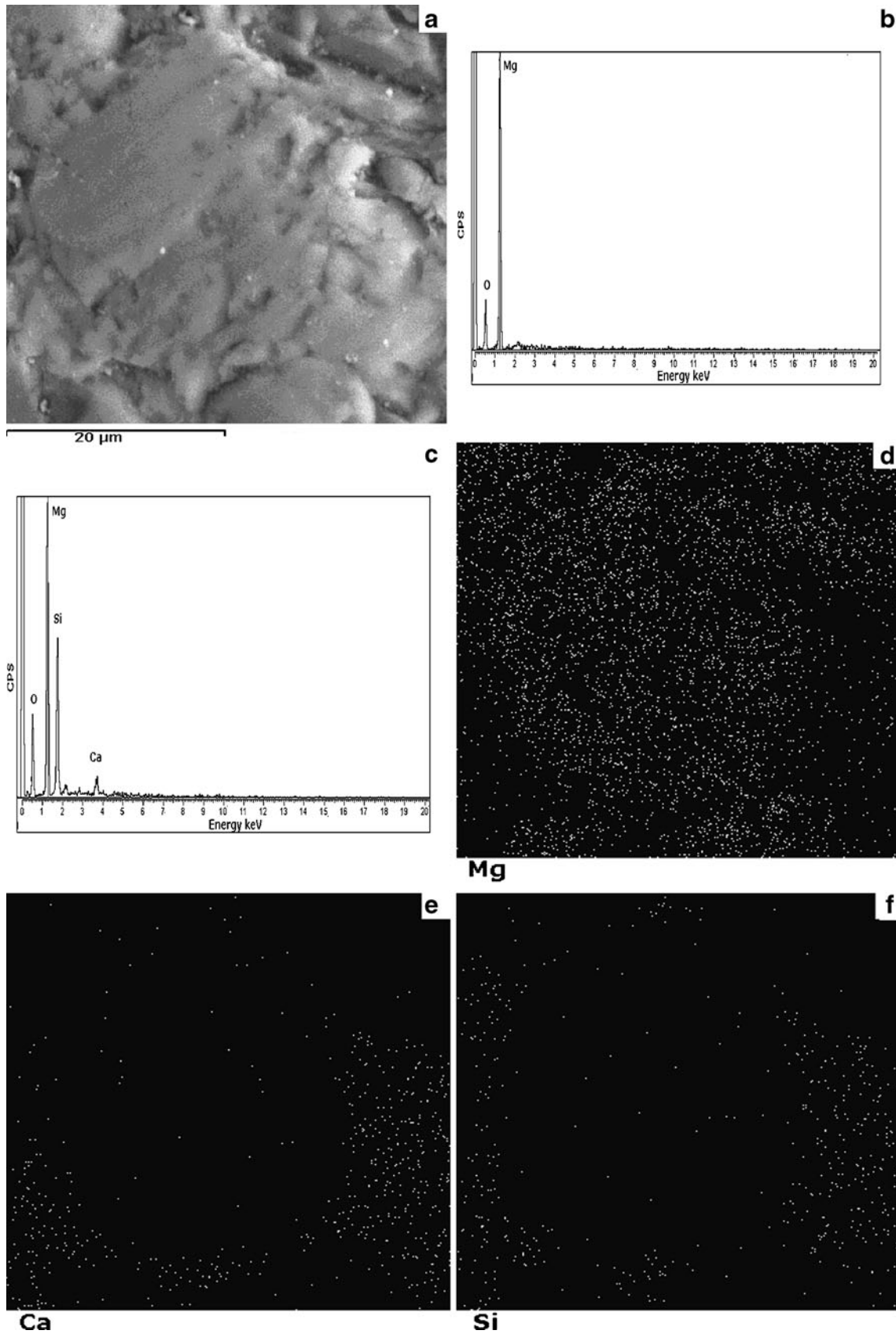
Figure 9. Scanning electron micrographs of AP1750 sample: (a) micrograph of an aggregate, (b) EDS analysis of the aggregate, (c) EDS analysis of the grain boundary, (d) Mg MAP elemental distribution, (e) Ca MAP elemental distribution and (f) Si MAP elemental distribution.
