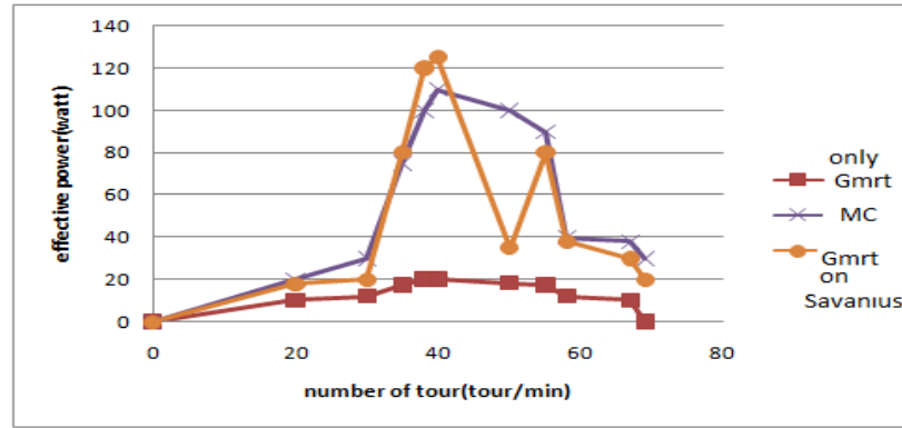
Figure5.Comparing effective power of gmrt and savonius
