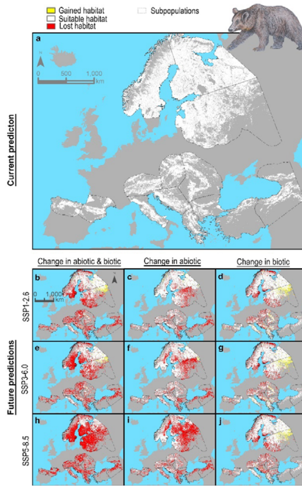
Fig. 4. Brown bear habitat predictions. a , Prediction of brown bear habitat for current conditions. Future predictions of habitat for climate change scenarios SSP1-2.6, SSP3-6.0 and SSP5-8.5 considering changes in both abiotic and biotic factors ( b , e , h ), changes in abiotic factors only ( c , f , i ) and changes in biotic factors only ( d , g , j ). The predicted area only includes a buffer area of 200 km around the current distribution to avoid extrapolating biotic variables into an environmental space where there is no information about the trophic interactions of brown bears.
