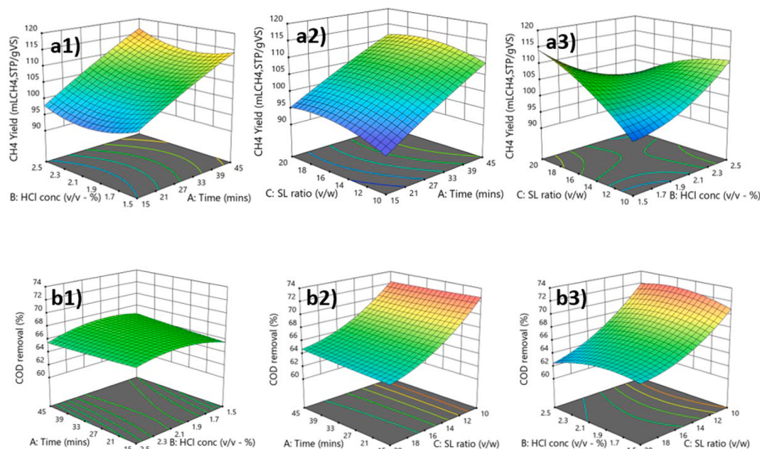
Fig. 4. Response surface plots for a) bio-CH 4 yield and b) COD removal .
