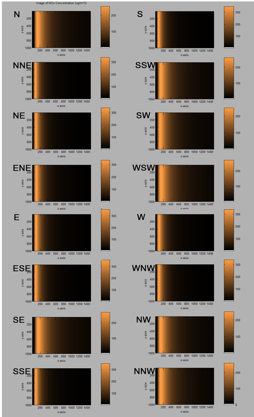
Figure 5. Dispersion profile of NO x pollutants during winter with slight insolation
